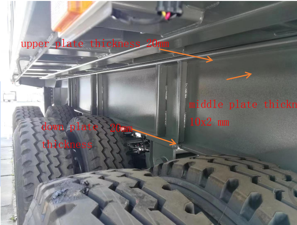
ZF truck trailer dumper trailer main beam
